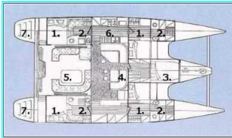
Boat Layout
